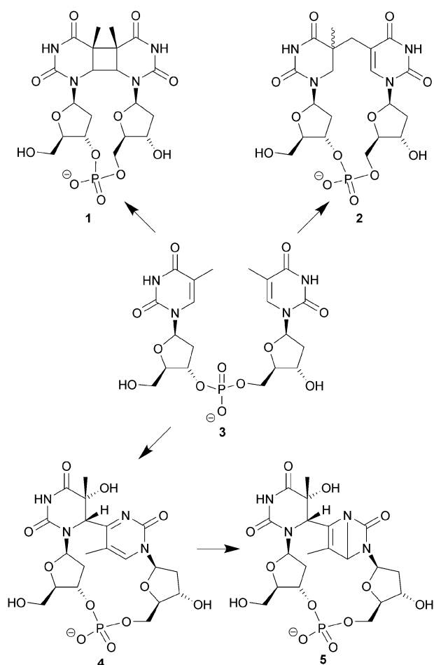
Scheme 1 Depiction of the four main pyrimidine-pyrimidine photolesions. 1: Cyclobutane pyrimidine dimer, 2: spore photoproduct, 4: (6-4) photoproduct, 5: Dewar valence isomer of 4 .
