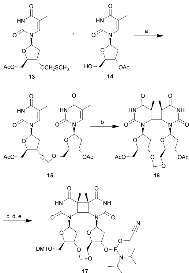
Scheme 3 Synthesis of T(CPD)T with formacetal backbone 17 , (a) NIS, TFOH, THF; (b) h\nu (150 W Hg-lamp), acetone; (c) NH 4 OH, rt, 12 h; (d) DMTCl, pyridine, DIEA; (e) (NCCH 2 CH 2 O)PN( i -Pr) 2 (Cl), DIEA, THF.
