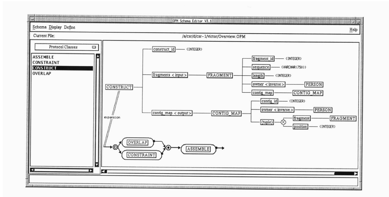
Figure 5: An OPM schema [15]
