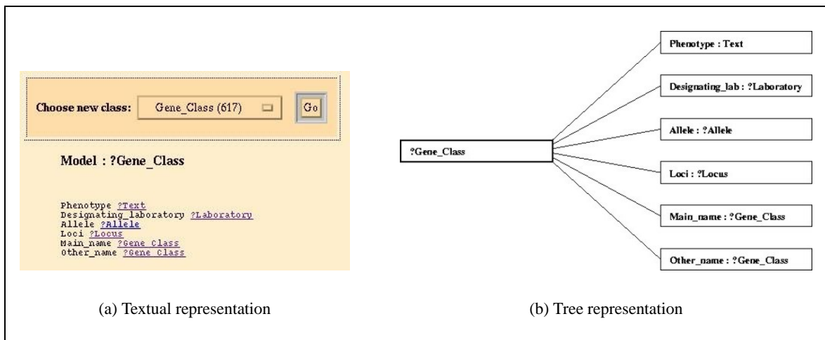
Figure 4: An ACEDB object (of the class “Gene_Class”) from the database ACeDB [22]
