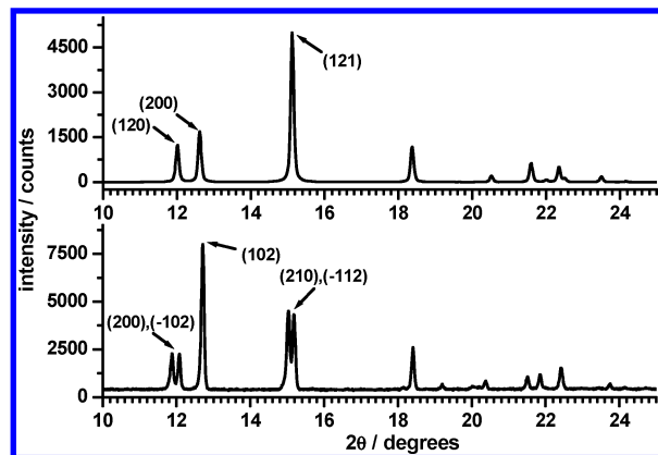
Figure 3. XRD patterns of \text{Cp}_3\text{Ho} ( \lambda_{\text{Cu K}\alpha} = 154.06 pm). The orthorhombic cell calculated from literature data 22 is depicted on the top. The monoclinic cell setting derived from the room-temperature measurement in our laboratory is depicted on the bottom.
