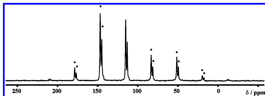
Figure 7. ^{13}\text{C}\{^1\text{H}\} CP MAS NMR spectrum of \text{Cp}_3\text{La} . Rotational sidebands of the isotropic chemical shifts \delta_{\text{iso}} are marked by asterisks.
