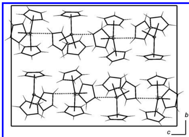
Figure 2. Projection of the unit cell of \text{Cp}_3\text{Ho} . View along axis a .
