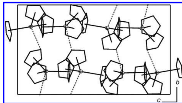
Figure 6. Projection of the unit cell of Cp 3 Ce along the unique axis a .
