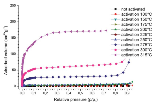
Fig. 10 \text{N}_2 adsorption isotherms at -196\text{ }^\circ\text{C} for {}^2_{\infty}[\text{Gd}_2\text{Cl}_6(\text{bipy})_3] \cdot 2\text{bipy} ( 1 ) in \text{cm}^3\text{ g}^{-1} uptake depending on the variation of the activation temperature of the MOF.
