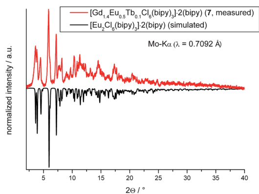
Fig. 1 Powder diffractogram of 7 (measured) compared to the powder diffractogram of the isotypic {}^2[\text{Eu}_2\text{Cl}_6(\text{bipy})_3]\cdot 2\text{bipy} (calculated).
