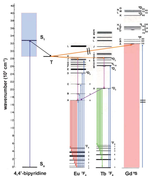
Fig. 9 Excitation and emission processes between metal ions and ligands in {}^2_{\infty}[\text{Gd}_{2-x-y}\text{Eu}_x\text{Tb}_y\text{Cl}_6(\text{bipy})_3] \cdot 2\text{bipy} ( 2–8 ).
