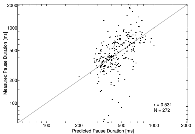
Figure 3: Scatter plot of predicted and measured pause durations of break index 4. Predictions are performed by linear regression based on Amplitude, F0, and logarithmic F0 reset.
