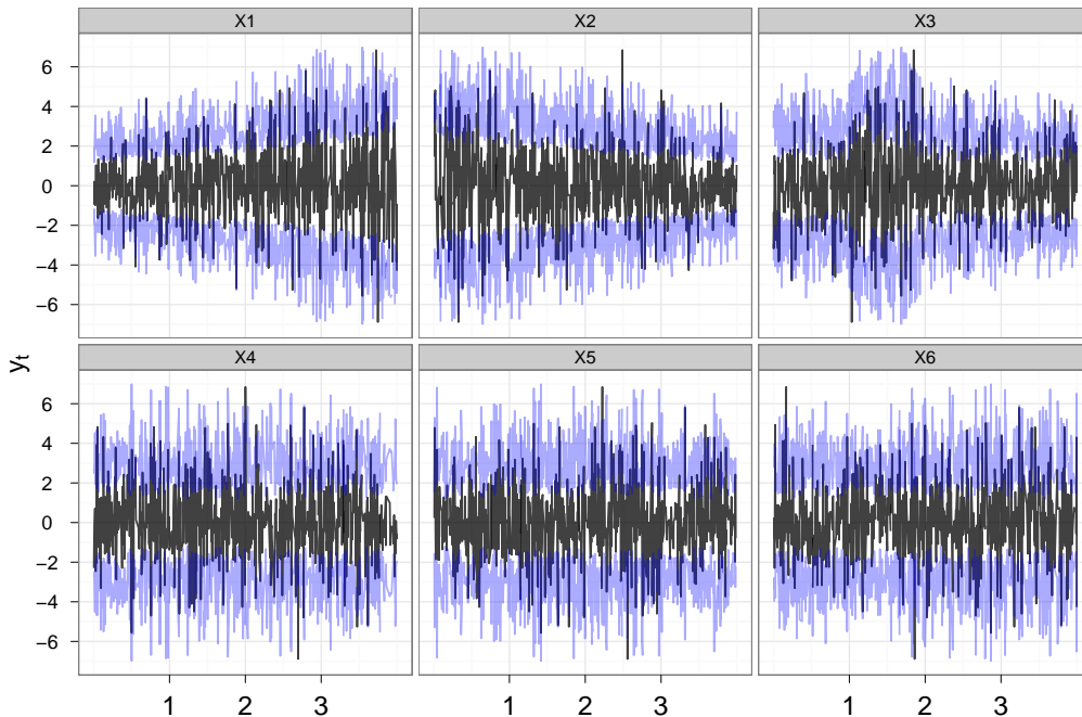
Figure 3: The observations y_t are depicted in black. The blue lines represent the 95%-interquantile range of the conditional density.
