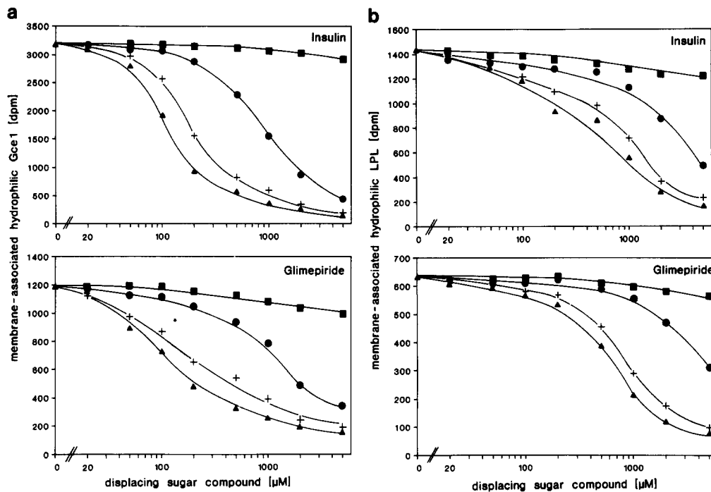
Figure 2. Dissociation from the membrane of lipolytically cleaved LPL and Gcel with sugar compounds. Adipocytes were metabolically labeled with myo -[ 14 C]inositol and subsequently incubated (30 min, 37°C) with insulin (10 nM) or glimepiride (10 μM). Plasma membranes were prepared, incubated (15 min, 4°C) in the absence or presence of the indicated concentrations of inositol-1,2-cyclic monophosphate (▲), inositol-1-monophosphate (+), glucosamine (●), and mannose (■) and then centrifuged through a cushion of sucrose. The plasma membranes recovered in the pellet were subjected to TX-114 partitioning. Hydrophilic Gcel (a) and LPL (b) were purified from the aqueous phase by affinity purification or immunoprecipitation, respectively. All samples were
