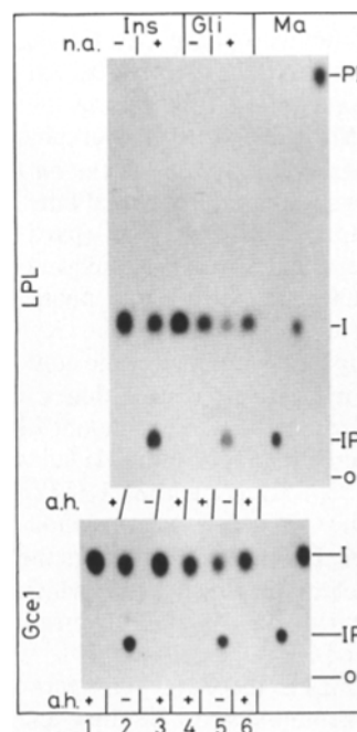
Figure 3. TLC analysis of the GPI anchor of hydrophilic LPL and Gcel. Adipocytes were metabolically labeled with myo -[ 14 C]inositol and subsequently incubated (30 min, 37°C) with 10 nM insulin ( Ins ) or 10 μM glimepiride ( Gli ). Plasma membranes were prepared and subjected to TX-114 partitioning. Hydrophilic Gcel and LPL were purified from the aqueous phase by affinity chromatography or immunoprecipitation, respectively, and then subjected to nitrous acid deamination ( n.a. ) or left untreated. The untreated and one half of the deaminated samples were hydrolyzed with HCl ( a.h. ), the other half was left untreated. All samples were analyzed by TLC and fluorography. The positions of radiolabeled markers, inositol-1-monophosphate ( IP ), myo -inositol ( I ) and phosphatidylinositol ( PI ), run in parallel, are indicated on the right margin ( Ma ).
