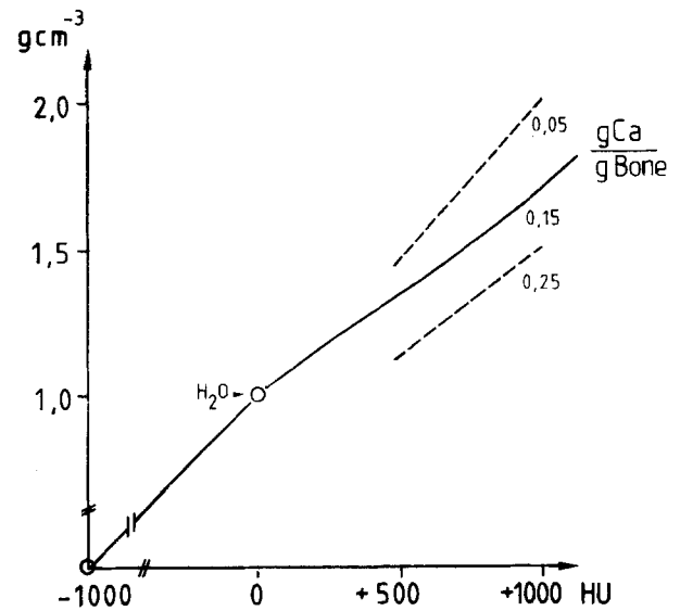
Fig. 6. Empirical relationship between values in Hounsfield units (HU) and physical density [21]
