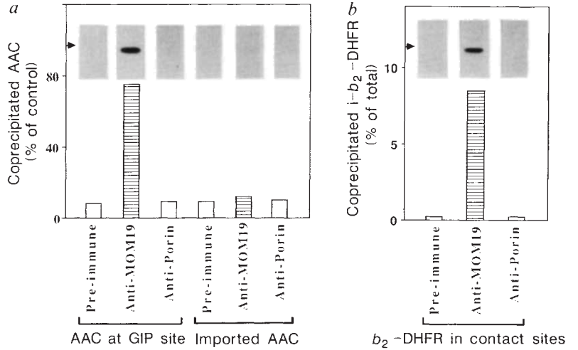
FIG. 2 Copurification of translocation intermediates with the receptor complex. a , Copurification of the GIP intermediate of ADP/ATP carrier. The arrowhead indicates copurified ADP/ATP carrier (AAC). b , Copurification of the contact site intermediate of b_2 -DHFR. The arrowhead indicates copurified intermediate-sized i - b_2 -DHFR.
