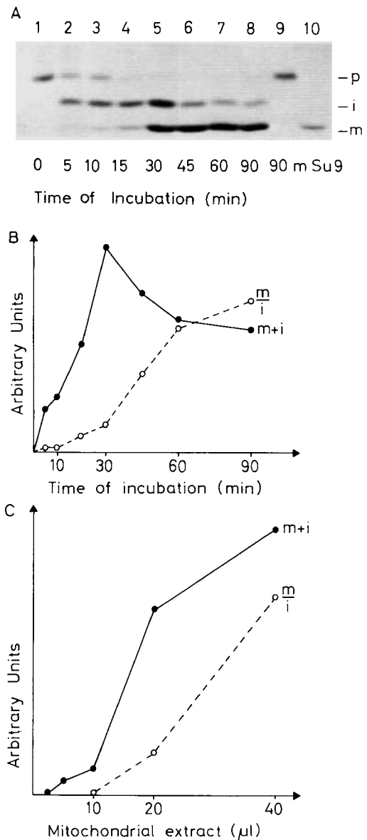
Fig. 1. Processing of the precursor to subunit 9 by a mitochondrial extract. (A) Aliquots of desalted lysate (100 \mu\text{l} each) containing radiolabeled precursors were incubated as described in Materials and Methods in a final volume of 225 \mu\text{l} with 20 \mu\text{l} of a mitochondrial extract for various time periods. Su 9 was immunoprecipitated and subjected to electrophoresis. Lane 9 contained no mitochondrial extract. Mature Su 9 (lane 10) was immunoprecipitated from mitochondria labeled in vitro . p, precursor; i, intermediate; m, mature Su 9 (B). The time course of processing shown in A was quantified by densitometry of exposed films. The values of m + i and m/i are plotted versus the time of incubation. (C) Aliquots of desalted lysate (100 \mu\text{l} each) were incubated as in A with the indicated amounts of mitochondrial extract for 1 h. Su 9 was immunoprecipitated and subjected to electrophoresis. Bands were quantified by densitometry of exposed films. The values of m + i and m/i are plotted versus the volume of mitochondrial extract
