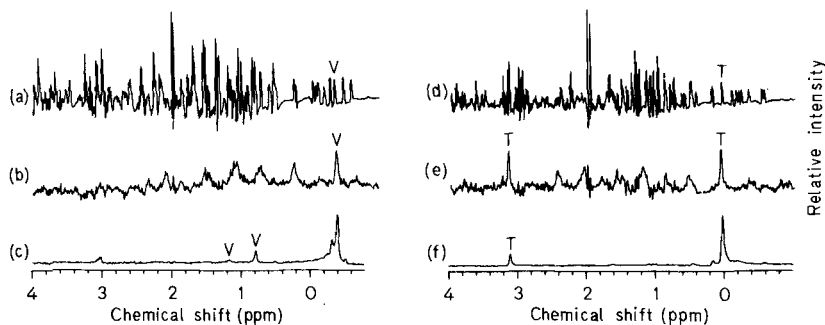
Fig. 6. 470-MHz NMR spectra of (a–c) tuna ferricytochrome c , 8 mM in ^2\text{H}_2\text{O} at pH 5.6 and 25°C; (d–f) horse ferricytochrome c , 8 mM in ^2\text{H}_2\text{O} at pH 5.6 and 25°C. (a) and (d) are resolution-enhanced spectra; (b) and (e) are the NOE difference spectra resulting from saturation of the resonance of haem methyl-5 at \approx 10 ppm for 1.5 s prior to application of the observation pulse; (c) is the NOE difference spectrum resulting from saturation of the \text{CH}_3 resonance of Val-28 at -0.46 ppm for 1.5 s prior to application of the observation pulse; (f) is the NOE difference spectrum resulting from saturation of the \text{CH}_3 resonance of Thr-28 at -0.01 ppm for 1.0 s prior to application of the observation pulse. Resonances of Val-28 of tuna ferricytochrome c and Thr-28 of horse ferricytochrome c are indicated by V and T respectively. The \text{CH}_3 resonances of thioether-4 occurs at \approx 3.1 ppm for horse [18] and tuna ferricytochromes c . These resonances may be affected by saturation of resonances of Val-28 and Thr-28 (c) and (f). The \beta\text{CH} resonance of Thr-28 overlaps with the \text{CH}_3 resonance of thioether-4
