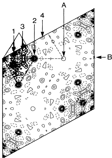
FIG. 4. Patterson function of the 6\times 6 superstructure. The shaded area corresponds to a \sqrt{3}\times\sqrt{3} unit cell. The interpretation of peaks 1–3 is given in Table V. At position B no peak is observed and the peak at position A is negligibly small.
