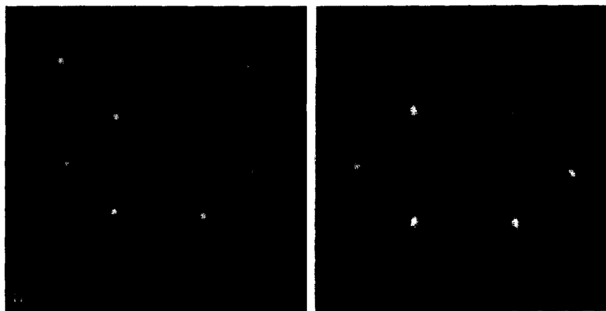
Fig. 1. LEED patterns of the clean Ta(100) surface: (a) at 310 K, 103 eV; (b) at 160 K, 77 eV.
