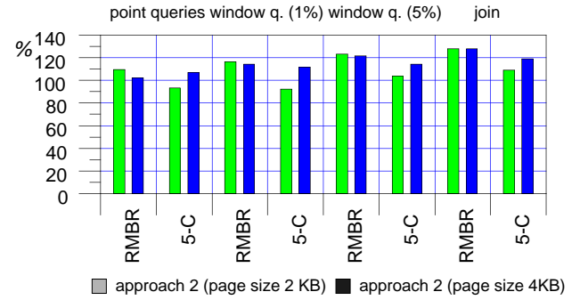
Figure 10: I/O-cost of approach 2 compared to approach 1
