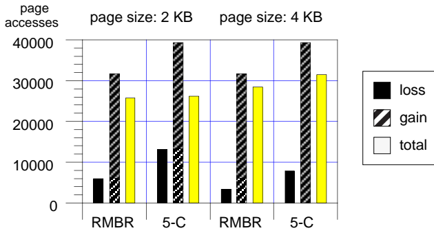
Figure 11: Change of performance using approximations
