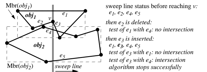
Figure 13: Example for the plane-sweep algorithm
