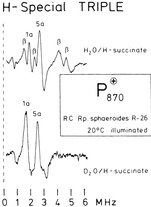
FIGURE 3 H-Special TRIPLE spectra of light-induced P\ 870^+ in solution; bacteria grown with protonated succinate in H_2O (top), and in 99.9% D_2O (bottom). Experimental conditions: total r.f. power 200 W, 4 scans, \pm 50 kHz fm deviation, rest as for ENDOR (Figure 2). The shoulders on lines 1a and 5a (bottom) are due to non-averaged hfs anisotropy of the methyl groups and not due to additional couplings. (The deuterated RC's were coagulated resulting in a considerable increased \tau_R value and solid state ENDOR line shapes.)
