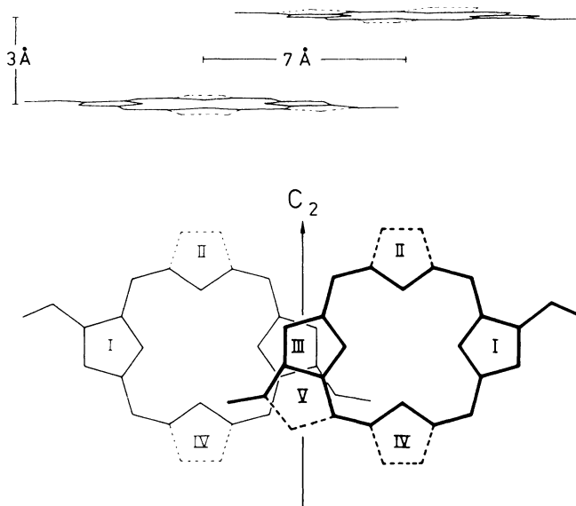
FIGURE 5 Horizontal and perpendicular view of the dimer model. Only the \pi -skeletons and the hydrated rings (broken lines) of the two monomeric halves are shown. Standard geometries with X-Ray modifications for the keto group at rings III were used for the Hückel MO calculations (CNDO/2 parametrization).
