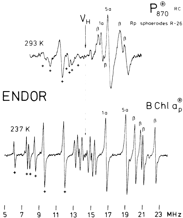
FIGURE 2 H-ENDOR-in-solution spectra of P\ 870^+ in RC's and BChl\ a_p^+ (both from Rp. sphaeroides R-26) at the given temperatures, the signs and assignments of the six largest hfc's (see Table I and II) are indicated. Experimental conditions, BChl\ a_p^+ : mw power 20 mW, r.f. power 100 W (11 G, rot. frame), 10 kHz fm of r.f. field, \pm 50 kHz deviation, no field modulation, time constant 1 s, 4 scans; P\ 870^+ : in situ illumination (450–900 nm, 500 W Xe high pressure lamp), mw power 80 mW, \pm 70 kHz fm deviation, 9 scans, rest as above.
