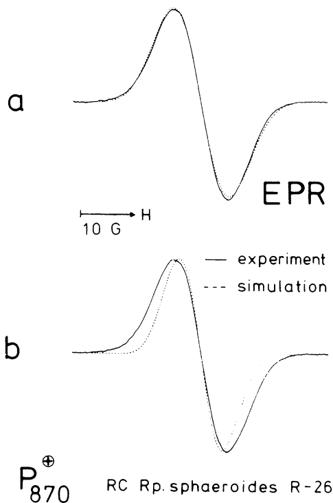
FIGURE 4 Experimental and simulated EPR spectra of P 870^+ in solution. For the simulation the ENDOR couplings and assignments from Table II were used; trace a: simulation assuming a dimer (twice the number of protons belonging to each hfc, linewidth 2.3 G obtained from the residual small hfc in P 870^+ and the ^{14}\text{N} couplings in \text{BChl } a^+ ); trace b: simulation assuming a monomer (linewidth 2^{1/2} \times 2.3 = 3.2 G).
