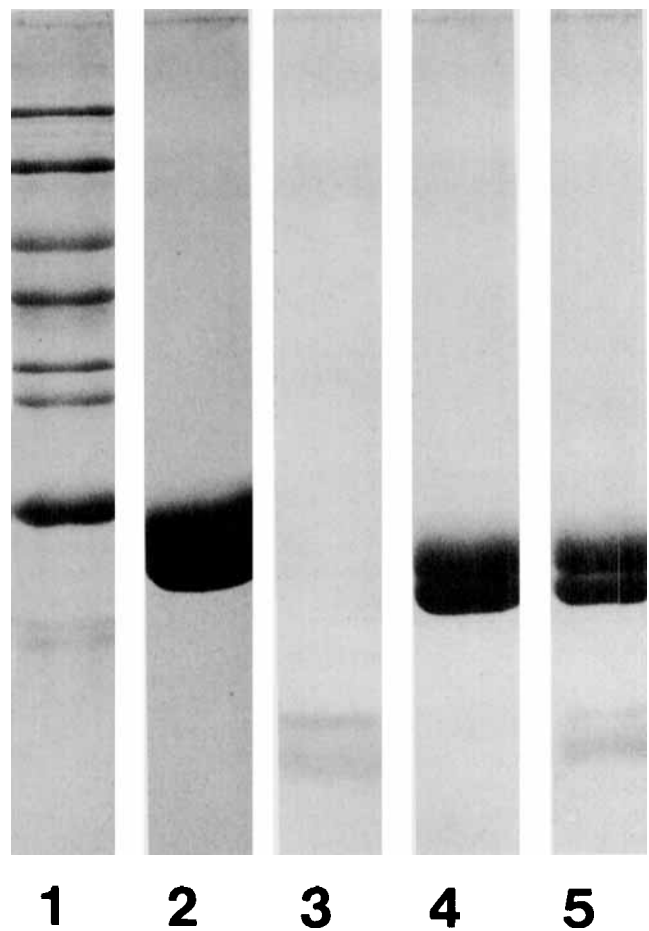
Figure 1. Sodium dodecyl sulfate PAGE of isolated polypeptides and reconstituted complexes. Lane 1, molecular weight markers (Sigma SDS VII-L marker kit: 14.2, 20.1, 24, 29, 36, 45, 66 kDa; plus \beta -galactosidase: 116 kDa); lane 2, AP as obtained from the TSK-DEAE column; lane 3, L_c^{8,9} as obtained from the S-Sepharose FF column; lane 4, reconstituted (\alpha^{AP}\beta^{AP})_3 complex; lane 5, reconstituted (\alpha^{AP}\beta^{AP})_3 \cdot L_c^{8,9} complex.
