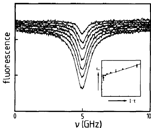
Fig. 1. A series of holes burnt at 1.6\text{ K} as a function of burning fluence. The laser intensity was 1.2\text{ }\mu\text{W}/\text{cm}^2 , burning times were between 80 and 1600\text{ s} . The inset shows the corresponding linewidth data ( \Gamma ) from which the quasi-homogeneous width \gamma ( 0.028\text{ cm}^{-1} ) was obtained by a linear extrapolation to zero fluence. The \Gamma scale is in units of 0.01\text{ cm}^{-1} , the I\tau scale in units of \text{mJ}/\text{cm}^2 .
