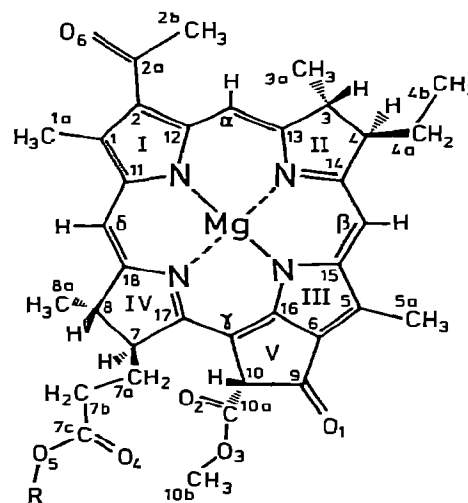
Fig. 1. Molecular structure of bacteriochlorophyll a. R = phytol (C 20 H 39 ) for R. sphaeroides .
