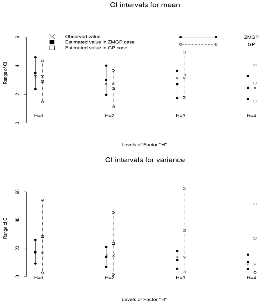
Figure 2: Confidence intervals (CI) for the mean (top panel) and variance (bottom panel) of the partial apple propagation data for ZMGP and GP models
