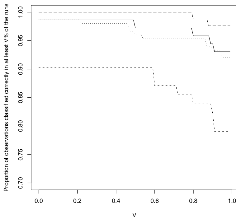
Figure 2: Survival plot for leukemia (solid), colon (dashed), SRBCT (long-dash) and iris (dotted).
