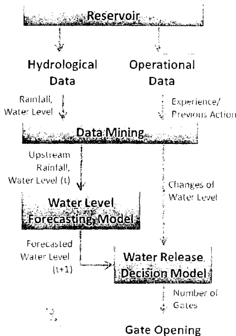
Fig. 5. Conceptual Model of IDSS for Reservoir Operation
