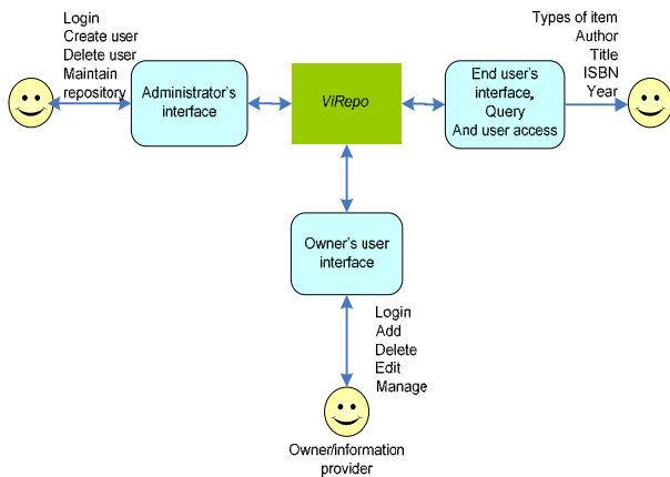
Figure 1: The context diagram showing the relationship between ViRepo with its three main entity
