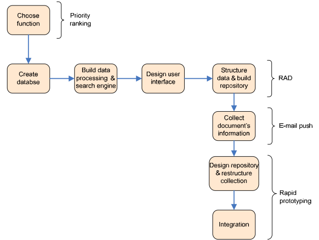
Figure 2: The process for building the ViRepo prototype
