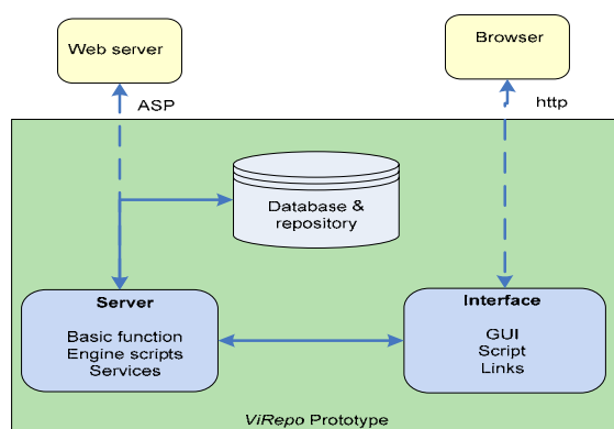
Figure 4: Components in the ViRepo architecture.
