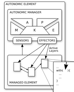
Fig. 9. MAPE-K architecture in context-oriented programming.
