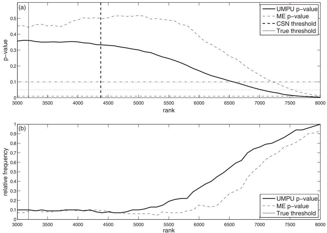
FIG. 7. (a) Average p -value (across 100 replications) for the ME and UMPU tests applied to the lognormal-Pareto mixture defined in (2). The dashed line represents the average x_{\min} identified by the CSN approach. (b) Relative frequency of replications for which the ME and UMPU tests reject the null hypothesis of Pareto for different thresholds.
