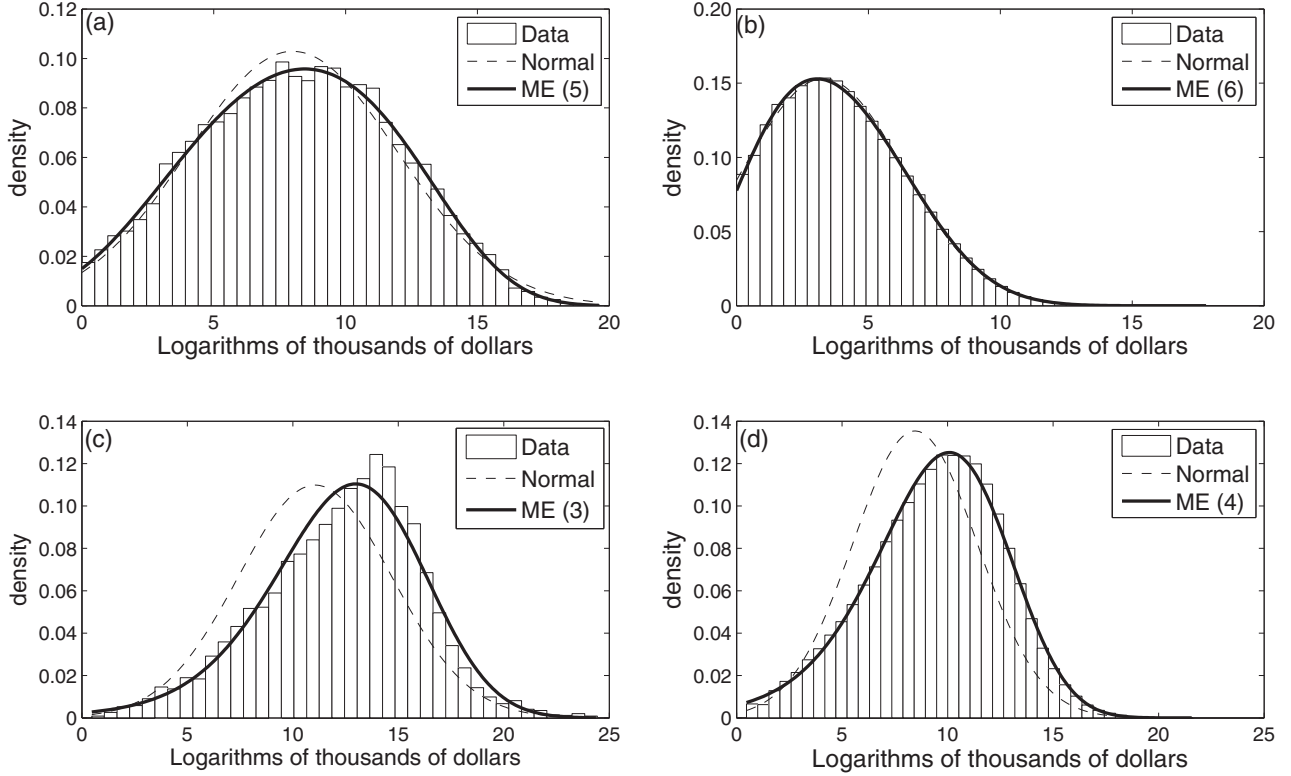
FIG. 2. Distributions of the logarithms of the data with superimposed the optimal ME density and the truncated normal density with parameters estimated from the data. From top to bottom and from left to right, the panels refer to aggregate trade data (a), disaggregate trade data (b), aggregate pharmaceutical data (c), and disaggregate pharmaceutical data (d).
