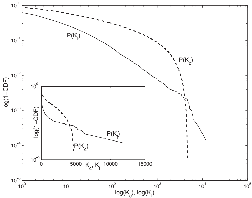
FIG. 6. The complementary cumulative distribution of the number of commodities traded by country pairs P(K_c) (trade data, broken line) and products by firm P(K_f) (pharmaceutical data, solid line). Double logarithmic scale (main figure) and semilogarithmic scale (inset).
