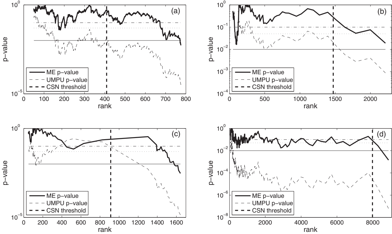
FIG. 3. The graphs show the (natural log of) p -value of the llr test for H_0 : k = 1 against H_1 : k = 2 in the ME setup, the estimate of x_{\min} obtained by CSN and the p -value of the UMPU test for exponential versus truncated normal. From top to bottom and from left to right, the panels refer to aggregate trade data (a), disaggregate trade data (b), aggregate pharmaceutical data (c), and disaggregate pharmaceutical data (d). The p -value of the CSN threshold is equal to 0.024 for aggregate trade, 0.274 for disaggregate trade, 0.026 for aggregate pharmaceutical, and 0.868 for disaggregate pharmaceutical data.
