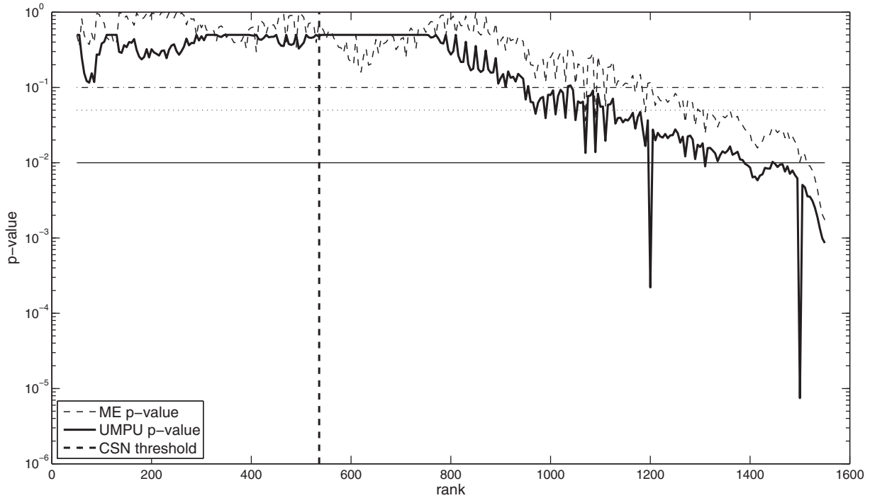
FIG. 1. (Natural log of) p -value of the UMPU and ME tests for exponential vs truncated normal distribution of the logarithm of US city sizes. The estimate of x_{\min} obtained by CSN is also reported (vertical line).
