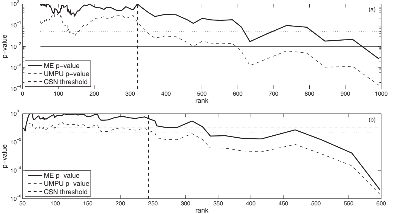
FIG. 5. Results for the length of the Pareto tail for the sampled trade (a) and pharmaceutical (b) data. The p -value of the Pareto tail found by means of the CSN approach is 0.096 for trade and 0.084 for pharmaceutical data.
