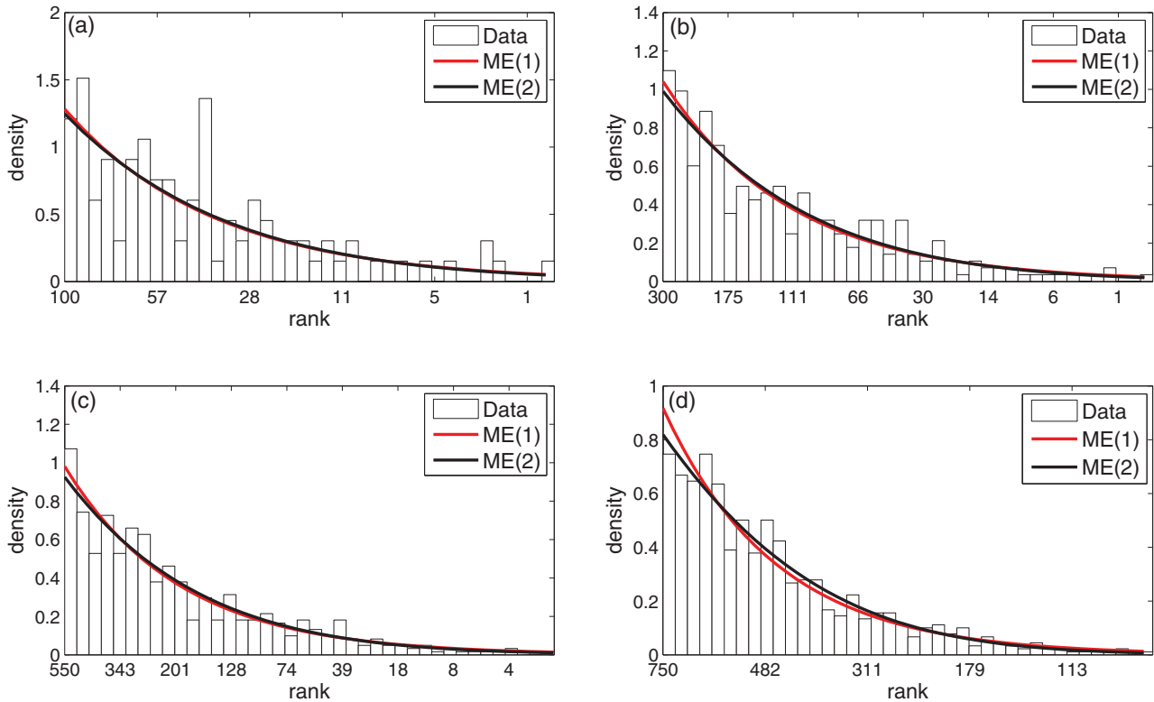
FIG. 4. (Color online) Results for the sampled aggregate trade data. ME(1) and ME(2) are the exponential and the truncated normal distribution, respectively.
