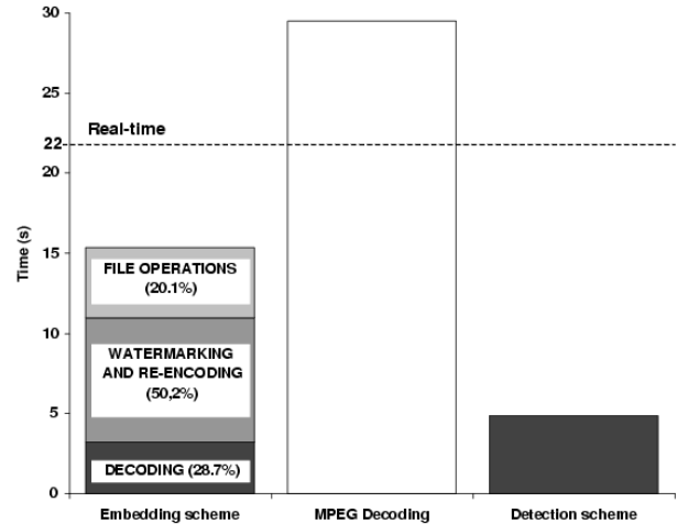
Fig. 4 Speed performance of the embedding and detection schemes.
