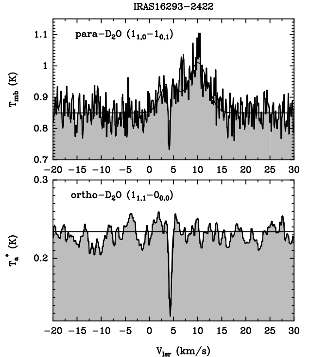
Fig. 2. Profile of the para-D 2 O ( 1_{1,0}-1_{0,1} ) line (histogram) observed at JCMT (upper panel), as well as the 3 component Gaussian fit (solid line) and ortho-D 2 O ( 1_{1,1}-0_{0,0} ) line observed with HIFI (bottom panel).
