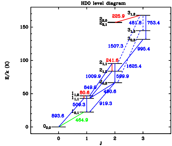
Fig. 1. Energy level diagram of the HDO lines. In red, IRAM-30 m observations; in green, JCMT observation; in blue, HIFI observations. The solid arrows show the detected transitions and the dashed arrows the undetected transitions. The frequencies are written in GHz.
