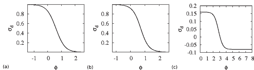
Figure 2. (a) and (b) Sketches of the adsorption isotherm from, respectively, the Langmuir and Frumkin–Fowler–Guggenheim models. 29 The parameters are Z = 3 , k_a^0/(k_a^0 C_b) = 1/6 and (a) \Delta G/RT = 0 , (b) \Delta G/RT = -2 , as used in ref 29. (c) Sketch of the adsorption isotherm for cobalt-hexamine on silica surfaces as given by eq 21. 19 In each figure, \sigma_d represents the surface charge density and \phi is the applied electrical potential.
