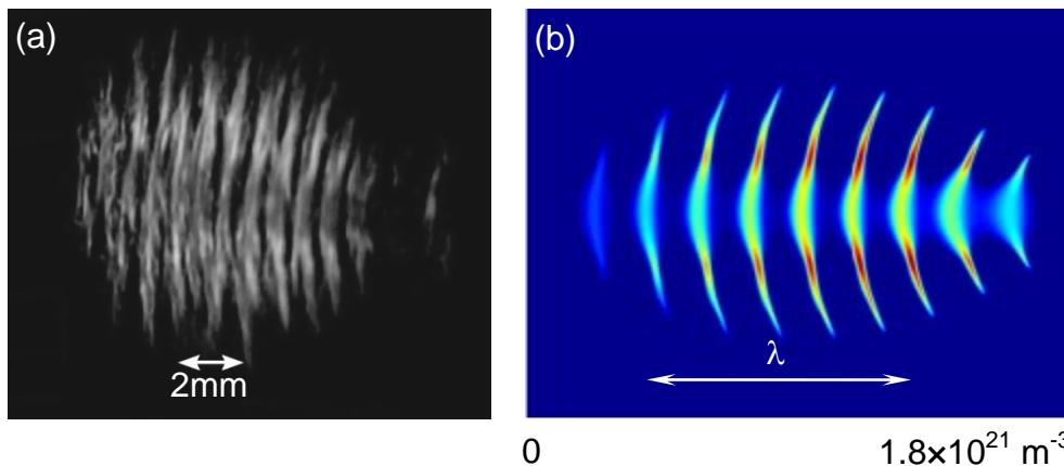
Fig. 4.8: (a) A typical experimental time-integrated volume breakdown plasma image in E plane under atmospheric pressure with incident amplitude 4.4MV/m ( 2.5\text{MW}/\text{cm}^2 in power density), 110GHz [1] . (b) Calculated distribution of the time averaged plasma density in the same conditions as Fig. 4.5.
