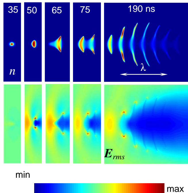
Fig. 4.6: Space distributions of the plasma density and electric field at different times. The colour scale for the density is between 0 and the maximum values: 0.04 , 1.7 , 3.3 , 4.2 , and 6.7 \times 10^{21} \text{ m}^{-3} for five successive times. The colour scale for the field is between the minimum and maximum values symmetric with respect to the incident rms field of 3.54 \text{ MV/m} within the intervals of [3.44, 3.64] , [2.54, 4.54] , [1.28, 5.28] , [0.48, 6.6] , and [0.0, 7.08] \text{ MV/m} for five successive times.
