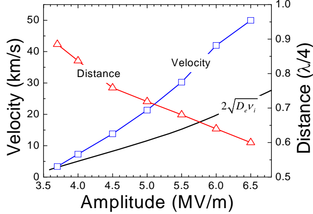
Fig. 3.10: Calculated average propagation velocity (square symbols) and distance between plasma filaments (triangle symbols) in unit of quarter wavelength as a function of incident microwave amplitude (110GHz). The velocity v = 2\sqrt{D_e v_{eff}} where v_{eff} is the effective ionization frequency calculated for the incident field is also plotted for comparisons (line).
