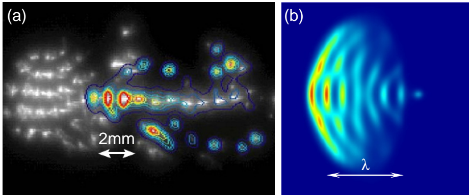
Fig. 4.5: (a) A typical microwave breakdown plasma images in H plane under pressure of 710 torr with incident power density 3.5\text{-}4\text{MW}/\text{cm}^2 ( \sim 5.4\text{MV}/\text{m} in amplitude, 110GHz), the black and white was captured by the slow camera (time-integrated values) and the pseudo colour was taken by the fast gated camera (instantaneous values) [2] . (b) Distribution of the plasma density in the same conditions of Fig. 4.3
