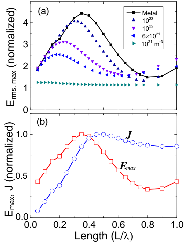
Fig. 5.10: (a) Calculated field (normalized by the antinode field) at the tip of a “plasma wire” (thickness \lambda/20 with given constant plasma density) as a function of its length normalized L/\lambda in the same arrangement as Fig. 5.2. The field calculated for a metal wire is also represented. (b) Electric field at the tip of a metal wire, and amplitude of the current flowing through the wire in its middle as a function of the wire length.
