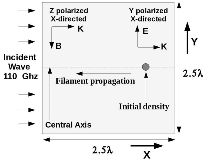
Fig. 4.1: Schematic of the computational problem and simulation domain ( X , Y ). Wave propagation is from left to right. Two cases are considered: Y -polarized, X -directed wave (electric field in the simulation plane), and Z -polarized, X -directed wave (electric field perpendicular to the simulation plane). Seed electrons are represented by an initial Gaussian density profile.
