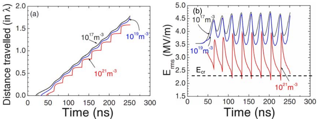
Fig. 4.10: (a) Positions of the plasma front as a function of time in the conditions of Fig. 4.5; the different curves correspond to different definitions of the plasma front, corresponding to different given values of the plasma density ( 10^{17} , 10^{19} and 10^{21} \text{m}^{-3} ), (b) rms electric field as a function of time at the same locations as (a), the critical value for rms field is also marked with dash line.
