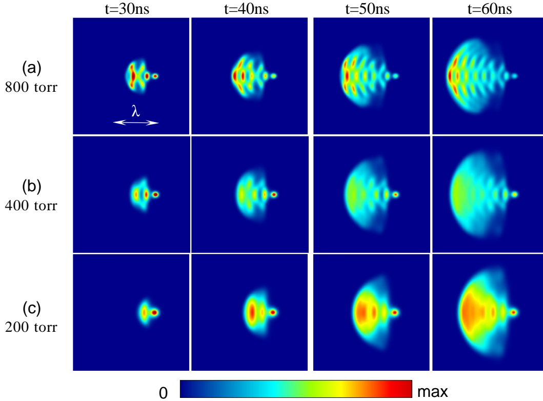
Fig. 4.14: Plasma pattern evolution for different 110GHz incident microwave with the same reduced incident effective field E_{eff}/p = 6.9 \times 10^3 \text{ V/m}\cdot\text{torr} for different pressure, and the coefficient for combination is \alpha=0.5 . The maximum density is 4.2 \times 10^{21} , 2.2 \times 10^{21} and 7.1 \times 10^{20} \text{ m}^{-3} for (a), (b) and (c), respectively.
