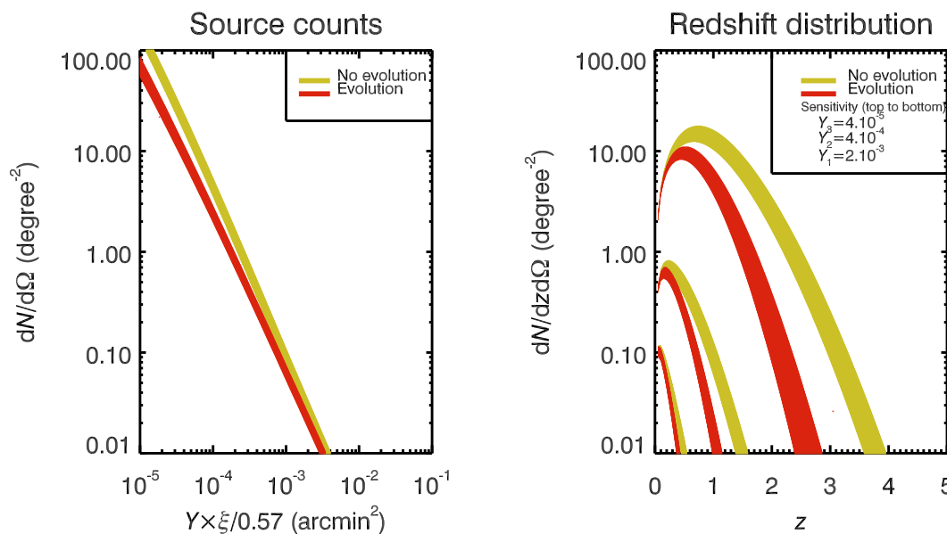
Fig. 2. Predicted galaxy clusters number counts detected from the Sunyaev-Zeldovich effect, after joint analysis of CMB, SNIa, LSS data and estimated temperature distribution function. Models describing self consistently the low and high redshift temperature distribution functions, needing non-standard evolution of T_X - M relation, lead to lower abundance of clusters, showing a deficit in the cluster number increasing with redshift ( right ). The best model being \Omega_m = 0.317 , \sigma_8 = 0.842 , h = 0.669 and A_{TM} = 7.31 .
