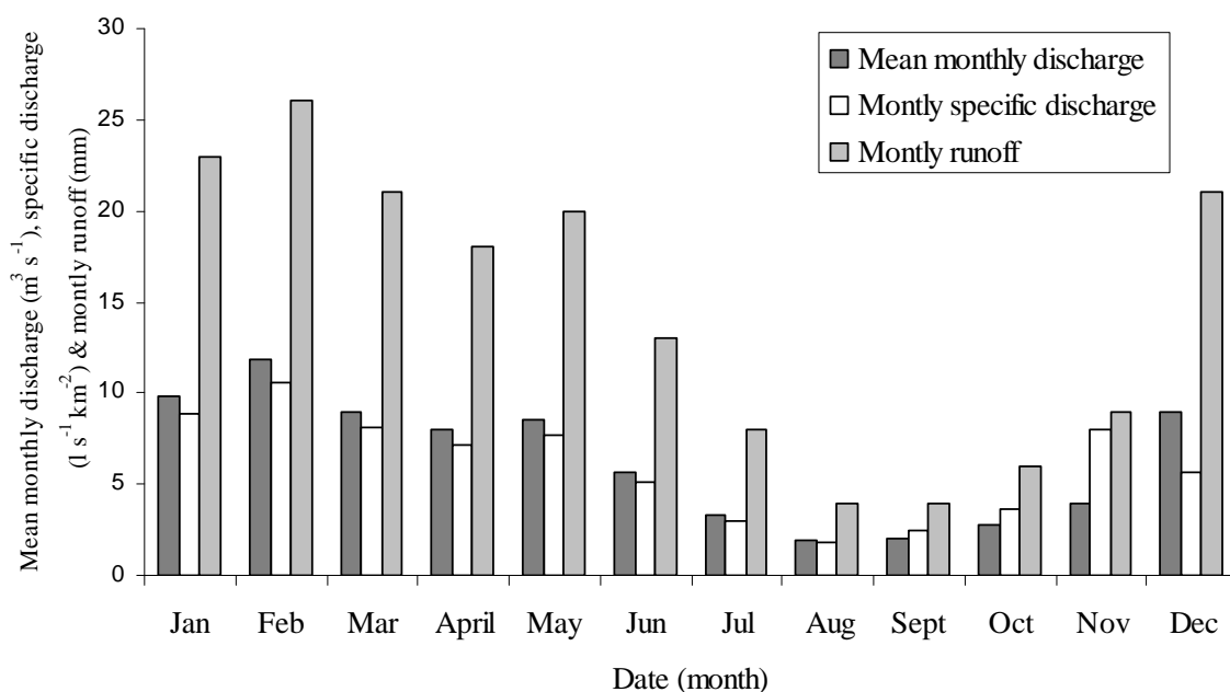
Figure 3-4: Summary of mean monthly discharge ( \text{m}^3 \text{s}^{-1} ), specific discharge ( \text{l s}^{-1} \text{km}^2 ) and runoff (mm) in the Save catchment at Larra gauging station (1965-2006) (Data from CAGG) (banque hydro http://www.hydro.eaufrance.fr/ )
