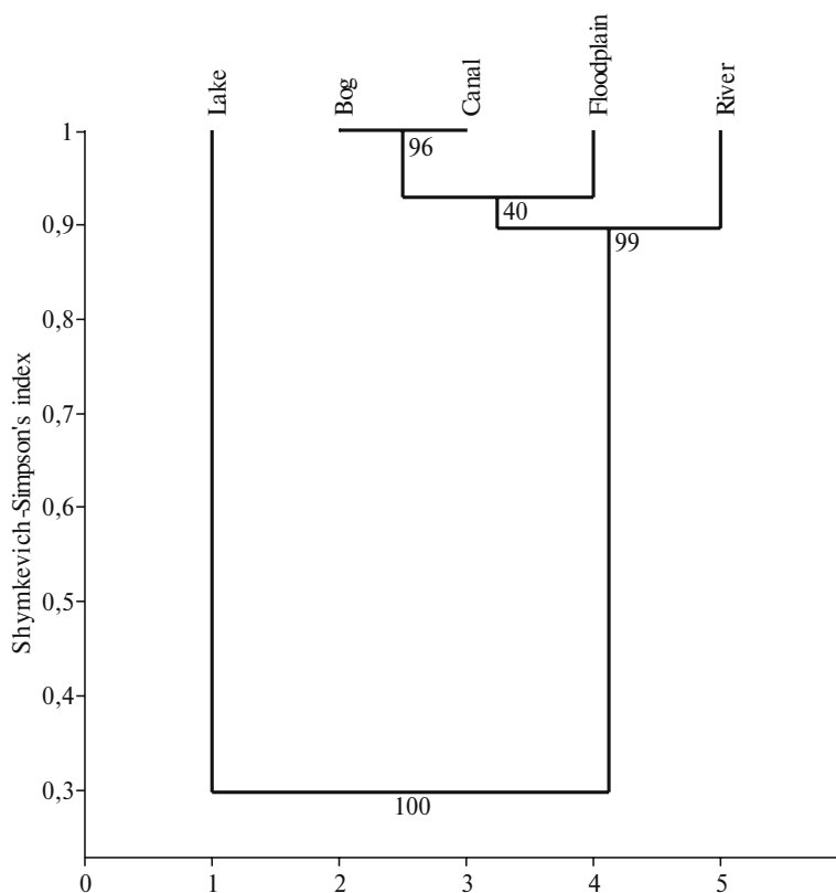
Fig. 3. The similarity between species compositions in different types of waterbodies regarding Szymkievich-Simpson index (in the nodes of dendrogram marked the probabilities of clusters (%) resulting Bootsrap analysis with 1000 repositions).
