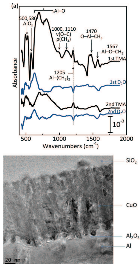
Figure 6. (a) Differential infrared absorbance spectra of CuO after alternative TMA and \text{D}_2\text{O} exposures up to 2 ALD cycles at 120 °C; (b) HR-TEM image of \text{Al}/\text{Al}_2\text{O}_3/\text{CuO} with 5 nm of \text{Al}_2\text{O}_3 .
