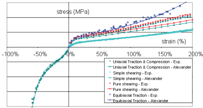
Figure 1. Comparison between Alexander's law and experimental elementary tests.
