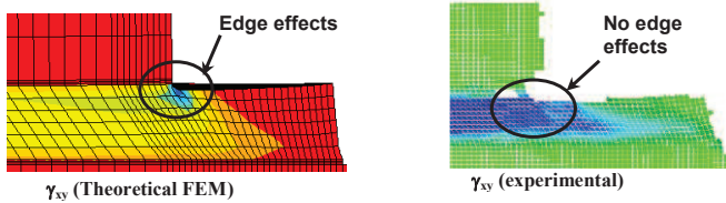
Figure 9. Theoretical (FEA) and experimental warping at end of connection.
