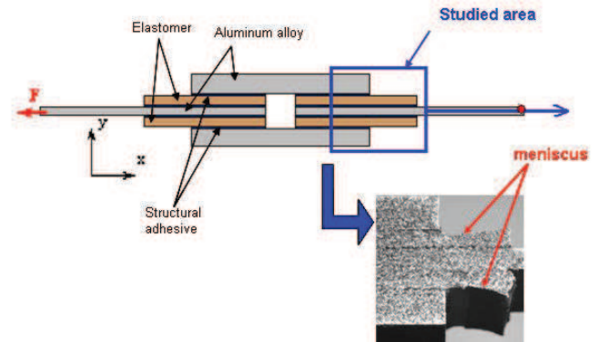
Figure 2. Quadruple shearing sample and studied area.
