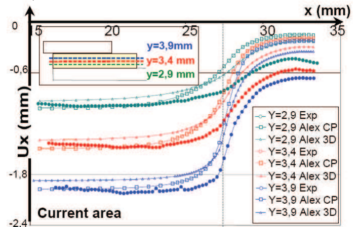
Figure 7. Comparison of FEA results in plane stress and in 3D.
