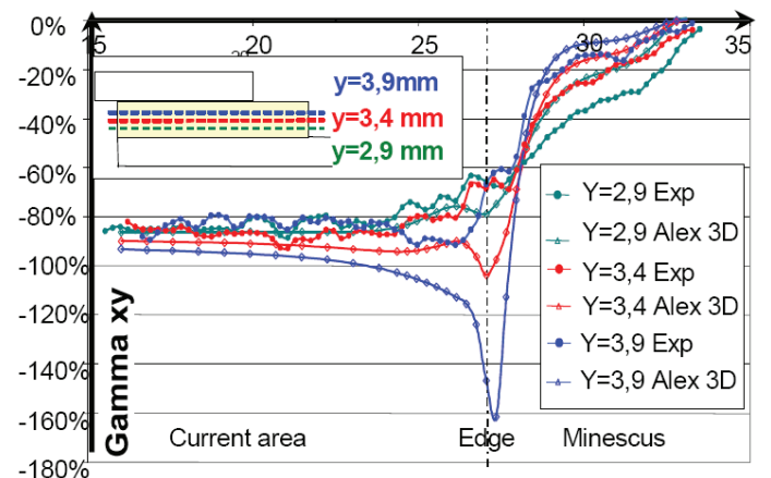
Figure 8. Theoretical (FEA) and experimental shear strain field.
