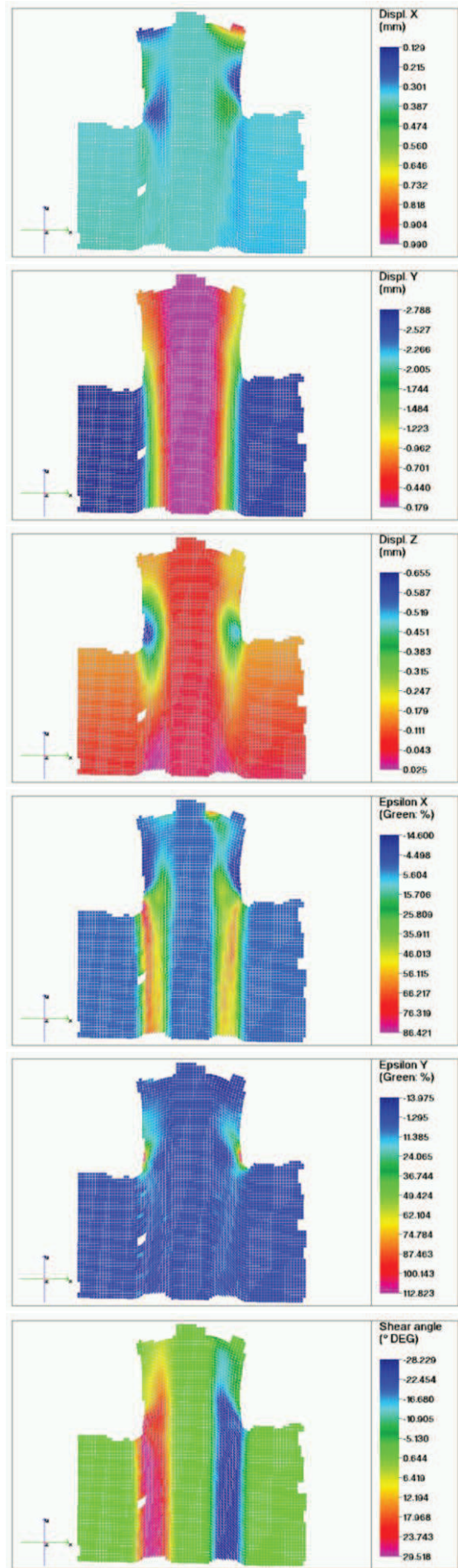
Figure 4. Experimental displacements and strain results for a theoretical warping of 100%.
