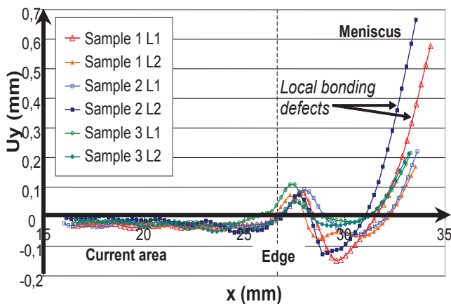
Figure 6. Superposition of the experimental results.
