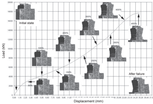
Figure 3. Load-displacement curve.
