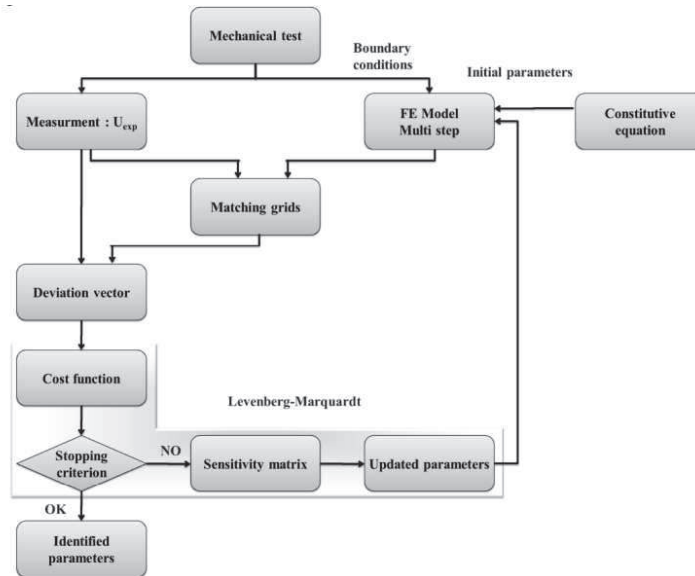
Figure 1: Identification procedure based on FEMU technique [3].
