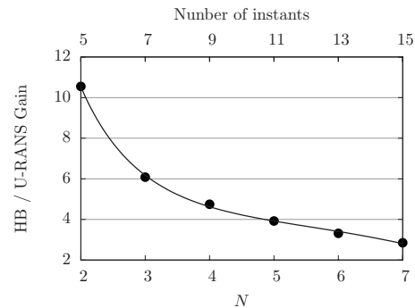
Fig. 15 HB computation CPU time gains
