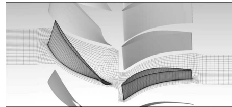
Fig. 2 CME2 Navier–Stokes wall-law mesh (one out of every two points)
