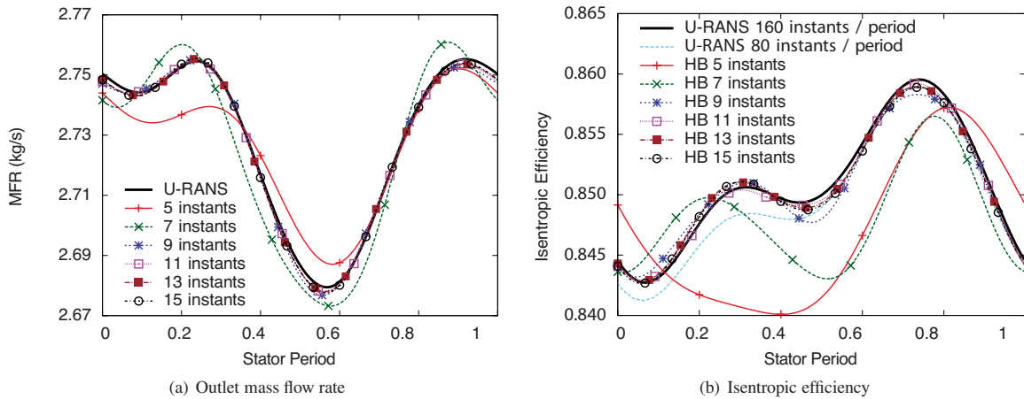
Fig. 7 HB computation MFR convergence (15 instants)
