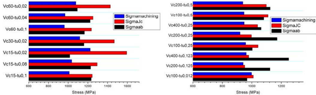
(a : Ti64) (b : Steel) Figure 4: Comparison between two identification methods
