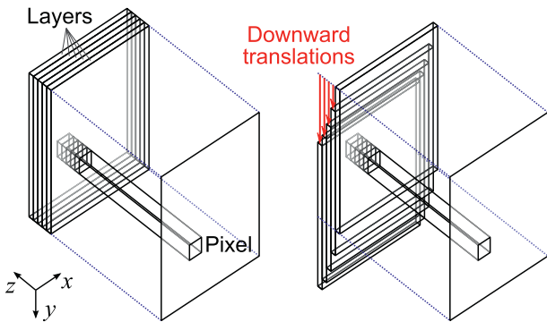
Fig. 5. In our model, the intensity of a pixel is obtained by integrating the fluorescein concentration carried by the layers. A downward translation (red arrows) is associated to each one of the layers for each one of the images of the input video. These translations are the unknowns of our problem. They are determined using our algorithm extending direct image registration.
