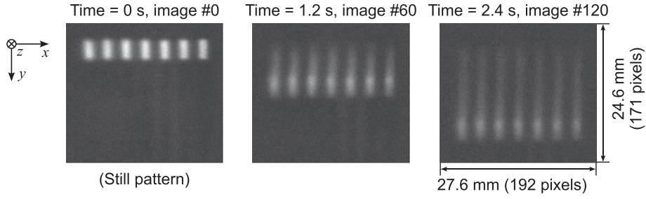
Fig. 7. Images extracted from the input video at three different instants. These are images after correction (in particular, they are negative version of the original ones). Image #0 is acquired when the liquid is still and it is used as the reference image. Images #60 and #120 are acquired when the Poiseuille flow is fully developed.
