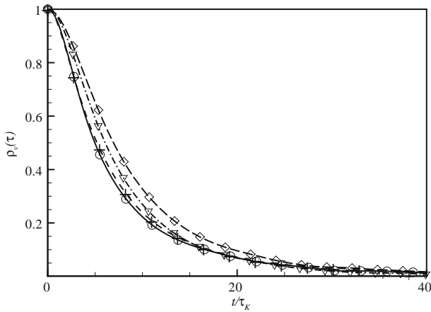
Fig. 7. Velocity auto-correlation function. Solid line with circles, B1; dashed line with crosses, B2; dash dot line with triangles, N1; long dash line with diamonds, S1.
