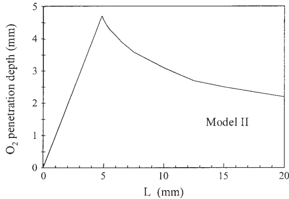
Figure 11. Example O 2 penetration depth ( \geq 0.1 \mu\text{M} concentration depth) predicted by Model 2 nitrification kinetics (Eq. 4b, 1^\circ \text{O}_2 , 1^\circ \text{NH}_4^+ ) as a function of sediment thickness (Model values as in Fig. 8, 9 and text). If higher levels of O 2 concentration are used to define penetration depth (e.g. \geq 10 \mu\text{M} ), similar relative patterns are obtained but the linear portion is contracted and maximum penetration depth occurs at a smaller L .
