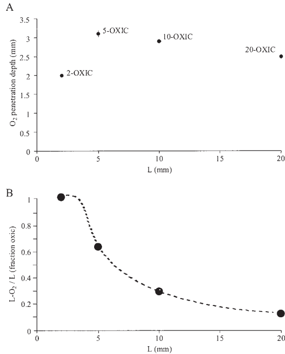
Figure 4. (A) Measured O 2 penetration depth (mean \pm SD) and (B) fraction of total plug thickness that is oxie as a function of plug thickness ( L ) (dotted line represents interpretive pattern).
