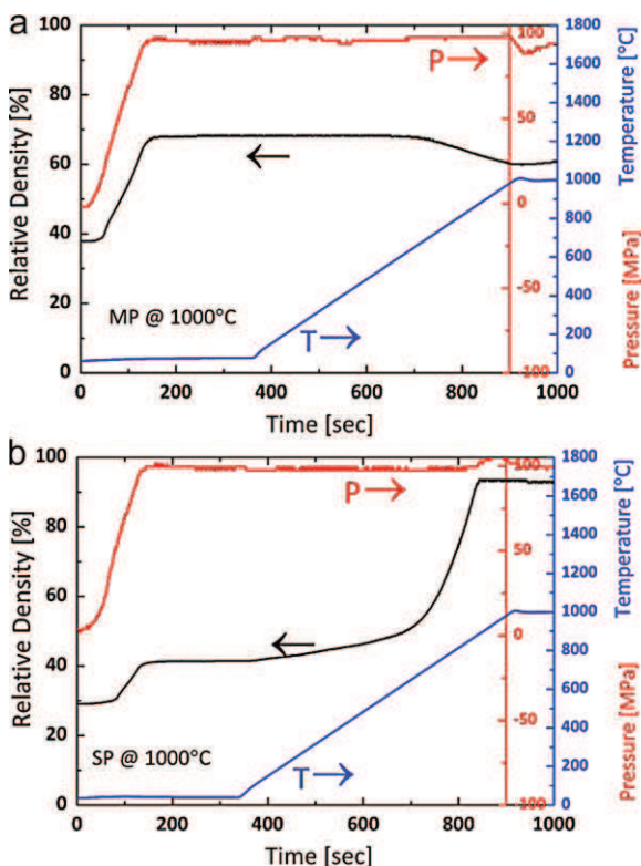
Fig. 4. Relative density–time–temperature–pressure dependencies during SPS of (a) MP and (b) SP Y_2O_3 nanoparticles at 1000^\circ C for 5 min and 100 MPa.
