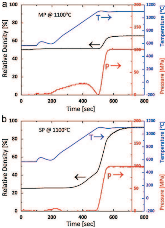
Fig. 5. Relative density-time-temperature-pressure dependencies during SPS of (a) MP and (b) SP Y_2O_3 nanoparticles at 1100^\circ C for 5 min and 100 MPa.
