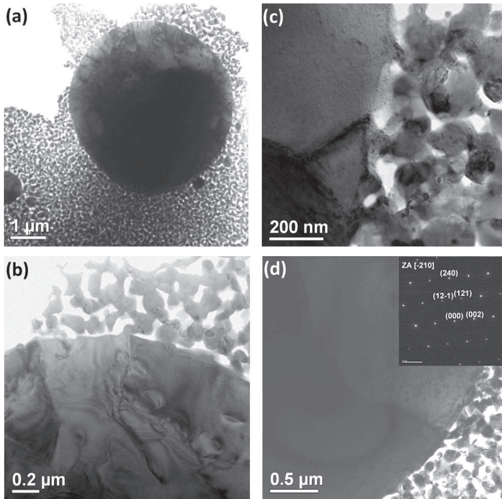
Fig. 8. TEM images showing the (a) nucleation and growth of the spherical cubic \text{Y}_2\text{O}_3 grains on account of the multiphase nanocrystalline matrix at 1000^\circ\text{C} . (b) Higher magnification of (a) showing the vermicular structure of the matrix nanoparticles. (c) The interface-controlled growth of the spherical cubic grains at 1100^\circ\text{C} . (d) Selected area diffraction pattern confirmed the cubic symmetry of the spherical \text{Y}_2\text{O}_3 grains.
