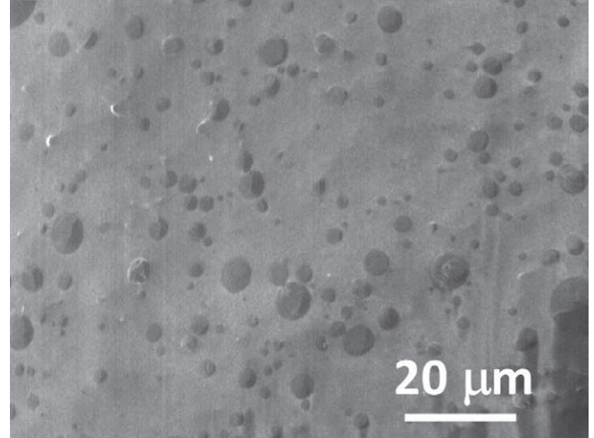
Fig. 7. SEM image showing the homogeneous distribution of the spherical grains throughout the specimen sintered at 1100^\circ C for 5 min and 100 MPa using multi-phase Y_2O_3 nanoparticles.
