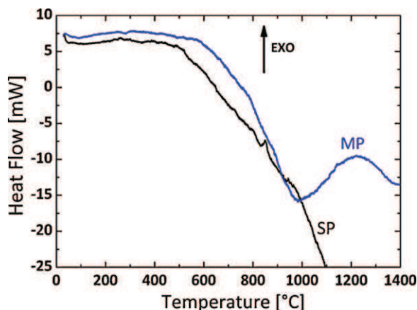
Fig. 3. Differential scanning calorimetry from nanocrystalline Y_2O_3 . (a) Single phase (SP) cubic. (b) Multiphase (MP) cubic + monoclinic.
