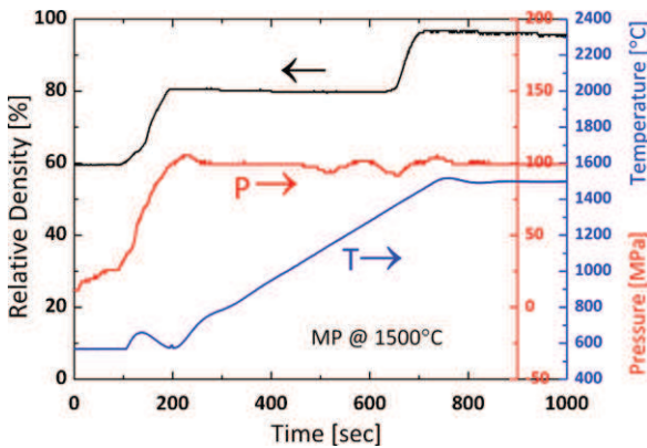
Fig. 6. Relative density-time-temperature-pressure dependencies during SPS of MP cubic Y_2O_3 nanoparticles at 1500^\circ C for 5 min and 100 MPa.
