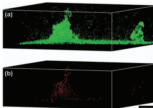
Figure 4. Viability of L. pneumophila cells in the biofilm. Images are volumic reconstructions of a 7-day-old biofilm of strain HW S2-14 (inoculum of 10^6 CFU ml -1 ) stained with Syto9 (a, total cells and eDNA) and PI (b, dead or damaged cells, eDNA). Scale bar = 50 \mu\text{m} .
