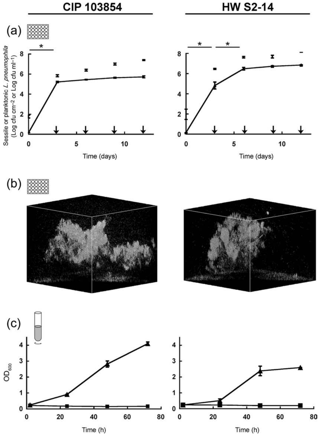
Figure 2. Growth of L. pneumophila (CIP 103854 on the left; HW S2-14 on the right) in SBB. (a) Kinetics of L. pneumophila biofilm formation ( \log [\text{cfu cm}^{-2}] , curve) and corresponding planktonic concentrations ( \log [\text{cfu ml}^{-1}] , dots) in microplate wells. Inocula consisted of 10^2 \text{ cfu ml}^{-1} . Bacteria were first quantified 2 h after inoculation. Arrows, medium renewal in microplate wells; bars, SD ( n = 3 ), * p -values \leq 0.01 between two biofilm quantification times. (b) L. pneumophila biofilm structures after 6 days. Images represent volumic reconstitutions of L. pneumophila biofilms observed with CLSM. Parallelepiped size is 375 \mu\text{m} \times 375 \mu\text{m} \times 284 \mu\text{m} for CIP 103854 and 375 \mu\text{m} \times 375 \mu\text{m} \times 265 \mu\text{m} for HW S2-14. (c) Planktonic growth of L. pneumophila in BYE ( \blacktriangle ) or SBB ( \blacksquare ) in tubes. Growth was monitored by the OD at 600 nm. Bars = SD ( n = 3 ).
