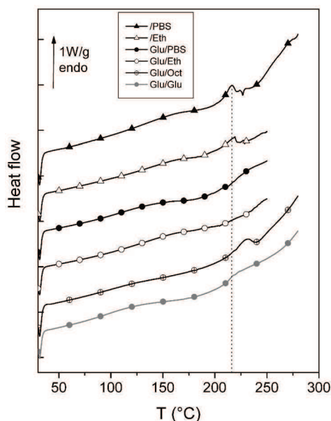
Figure 3. DSC thermograms of bovine pericardium samples in the dehydrated state recorded at 20\text{ }^\circ\text{C/min} from 30 to 250 or 280\text{ }^\circ\text{C} .
