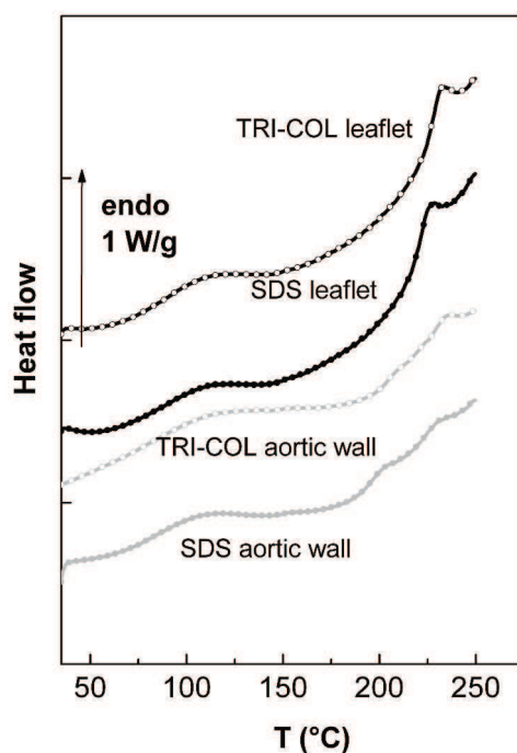
Figure 6. DSC thermograms of freeze-dried porcine aortic tissues (TRI-COL and SDS treated tissues) recorded between 40 and 250 °C recorded after a first scan performed between 40 and 150 °C.
