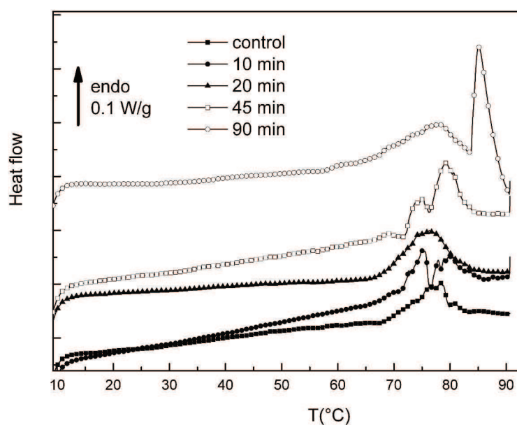
Figure 5. DSC thermograms of hydrated collagens (control and plasma jet treated collagens recorded at 10 °C/min between 10 and 90 °C.
