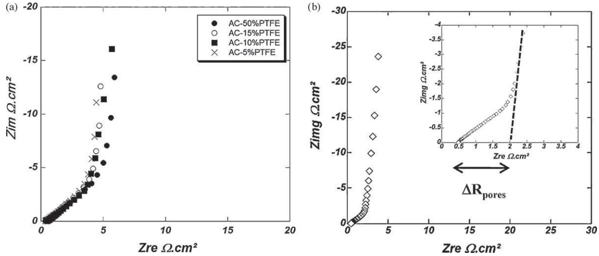
Fig. 6. Nyquist plots of SPS cell (a), of standard cell – AC-5%PTFE (b). Inset: determination of the ionic resistance of the electrolyte inside the porous carbon \Delta R_{\text{pores}} .
