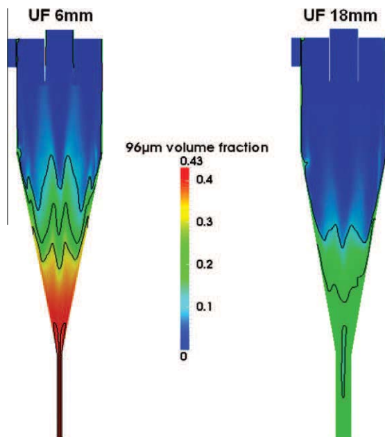
Fig. 18. Influence of spigot diameter on 96 µm diameter particles.
