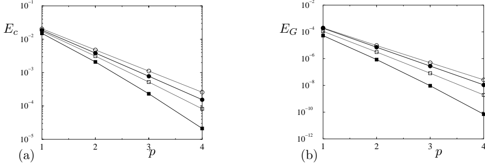
FIG. 4.3. Relative error for axisymmetrical N = 0 eigenmode. (a) Relative error E_c = |c_{\lambda_{0,p}^{\mathcal{D}}} - c_{l_{0,0}^{\mathcal{D}}}|/c_{l_{0,0}^{\mathcal{D}}} between the predicted amplitude and its theoretical value associated with a uniform initial temperature T_0 = 1 at z = 0 for the first Dirichlet eigenmode, versus the order p of the approximation. (b) Absolute error E_G = \|\Gamma_{\lambda_{0,p}^{\mathcal{D}}} - G_{l_{0,0}^{\mathcal{D}}}\| = \langle w(\Gamma_{\lambda_{0,p}^{\mathcal{D}}} - G_{l_{0,0}^{\mathcal{D}}})^2 \rangle on the predicted eigenfunction for the first Dirichlet eigenmode.
