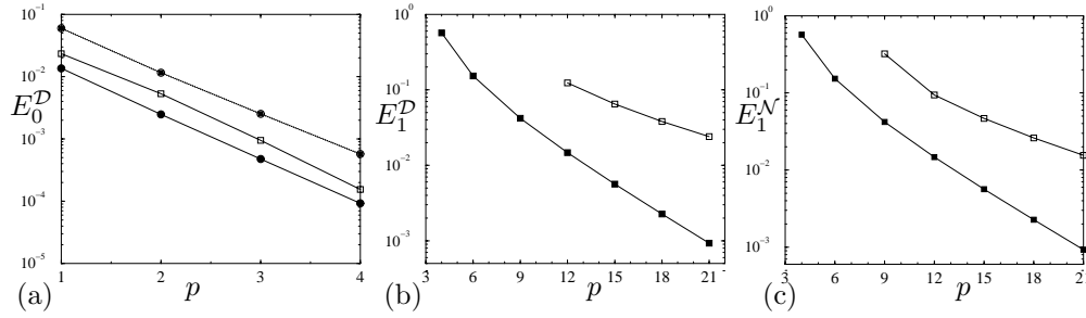
FIG. 4.2. Relative error for axisymmetrical N = 0 eigenvalues l_{0,0} and l_{0,1} . (a) Relative error E_0^D = |\lambda_{0,p}^D - l_{0,0}^D|/|l_{0,0}^D| between the predicted eigenvalue and the theoretical one l_{0,0}^D = -3.656793458 , versus the order p of the approximation. Black circles stand for the flow-averaging method with w = v/\langle v \rangle , and white circles for the classical uniform volume averaging w = 1 . White squares are for w = 1/(2r) and black squares are for w = 10(1-r)^3 . In every case the convergence is exponential, as indicated by the observed semilog linear behavior. (b) We use the same conventions for the second Dirichlet eigenvalue l_{0,1}^D = -22.30473055 convergence E_1^D = |\lambda_{1,p}^D - l_{0,1}^D|/|l_{0,1}^D| . (c) We use the same conventions for the second Neumann eigenvalue convergence l_{0,1}^N = -12.8398060 with E_1^N = |\lambda_{1,p}^N - l_{0,1}^N|/|l_{0,1}^N| .
