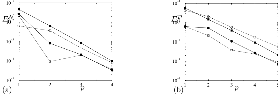
FIG. 4.4. We use the same conventions as in Figure 4.2 for the relative error for nonaxisymmetrical N = 1 eigenvalues l_{1,0} . (a) Relative error E_0^{\mathcal{N}} = |\lambda_{0,p}^{\mathcal{N}} - l_{1,0}^{\mathcal{N}}|/l_{1,0}^{\mathcal{N}} between the predicted eigenvalue and the theoretical Neumann one l_{1,0}^{\mathcal{N}} = -4.160532810 , versus the order p of the approximation. (b) We use the same conventions for the first Dirichlet eigenvalue convergence l_{1,0}^{\mathcal{D}} = -10.691151115 with E_0^{\mathcal{D}} = |\lambda_{1,p}^{\mathcal{D}} - l_{1,0}^{\mathcal{D}}|/l_{1,0}^{\mathcal{D}} .
