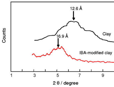
Fig. 4. X-ray diffraction spectra of (black) clay and (red) IBA-modified clay. (For interpretation of the references to colour in this figure legend, the reader is referred to the web version of the article.)
