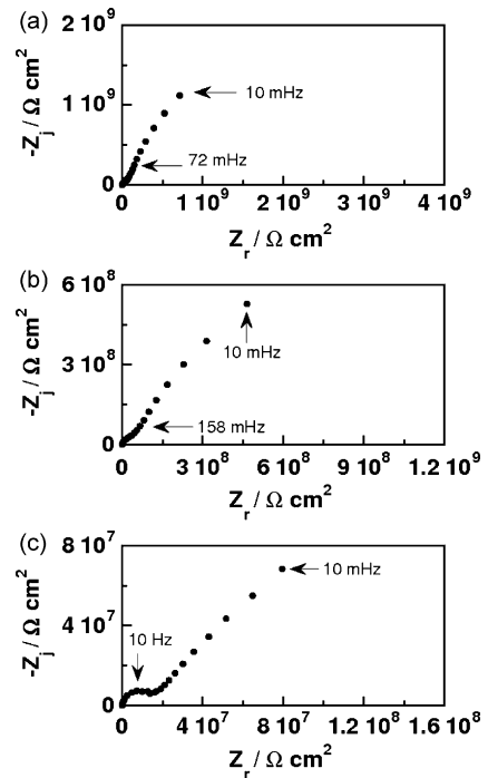
Fig. 7. Electrochemical impedance diagrams obtained for the carbon steel covered by the epoxy coating containing 2 wt.% IBA-modified clay after (a) 7 days (b) 14 days, (c) 56 days of exposure to 0.5 M NaCl solution.
