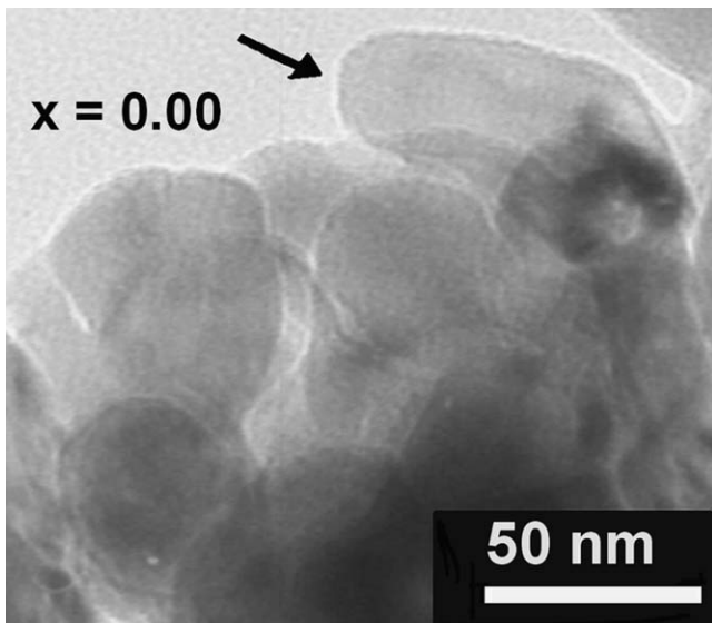
Fig. 4. Bright field TEM image of an undoped BTO powder sample showing grains which are in majority equiaxed ( D_{\text{average}} value = 54\text{ nm} ). Elongated grain is marked by an arrow.
