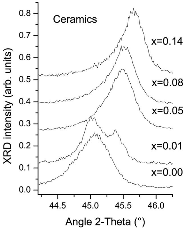
Fig. 3. XRD patterns of \text{Ba}_{1-x}\text{La}_x\text{TiO}_{3-\delta} ceramics with x=0, 0.01, 0.05, 0.08 and 0.14 , sintered at 1050\text{ }^\circ\text{C} , for 44.25^\circ < 2\theta < 46.25^\circ showing the splitting of (002) and (200) peaks and showing the decrease of the tetragonality (i.e., the decrease of the magnitude of the peak splitting) with increasing La content.
