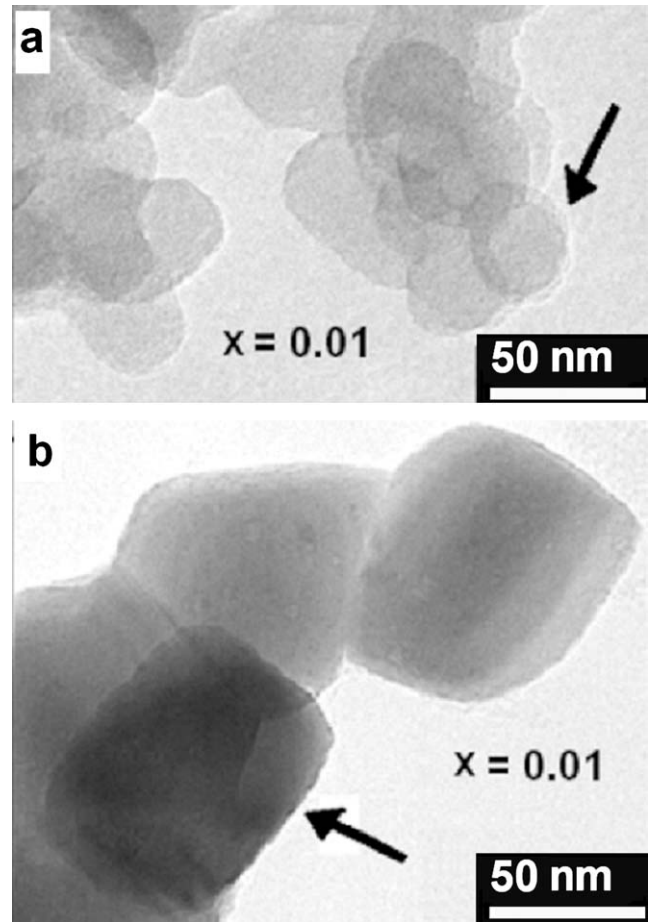
Fig. 5. Bright field TEM images of \text{Ba}_{1-x}\text{La}_x\text{TiO}_3 powder samples ( x=0.01 ) showing: (a) spherical shaped grains, as the grain marked by an arrow, and with GS value \sim 27\text{ nm} ; (b) tetragonal (close to quasi-cubic) and cubic shaped grains, as the grain marked by an arrow, and with GS much higher than those shown in (a).
