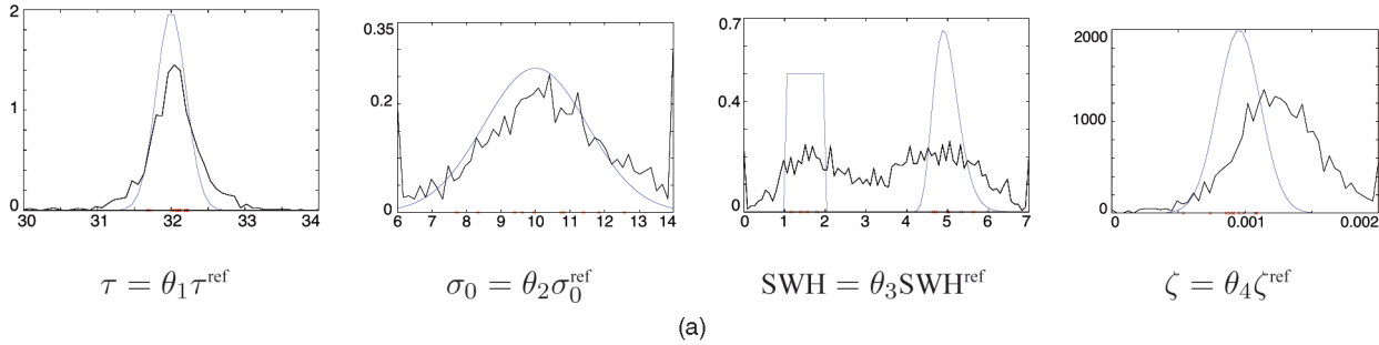
Fig. 5. Histograms of the four components of the parameter vector computed from the samples \tilde{\theta}^{(l)} for l \in \{3,001, \dots, 5,000\} (jagged lines), and pdfs used to sample the four components of the parameter vector (smooth lines). The crosses represent the values used in the simulations.
