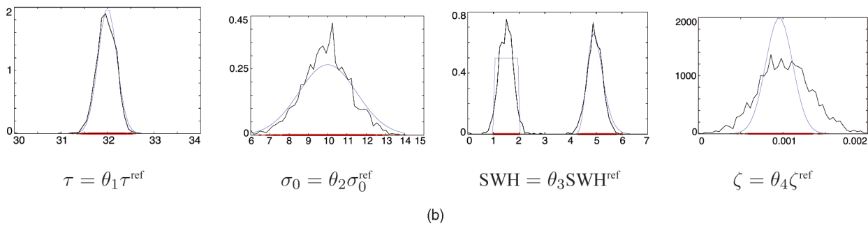
Fig. 6. Histograms of the four components of the parameter vector computed from the samples \tilde{\theta}^{(l)} for l \in \{3,001, \dots, 5,000\} (jagged lines), and pdfs used to sample the four components of the parameter vector (smooth lines). The crosses indicate the values used in the simulations. The number of training data is (a) N = 10 and (b) N = 1,000 (bottom row).
