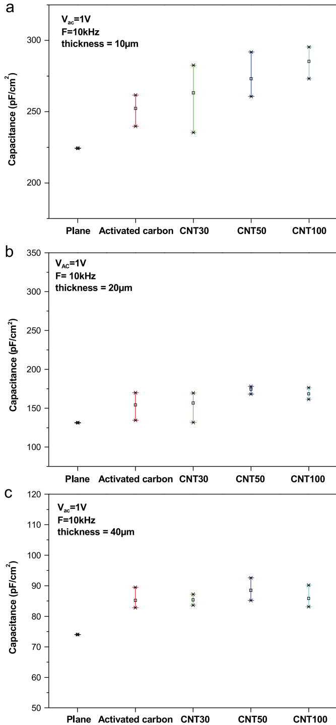
Fig. 2. (a) Capacitance values versus carbonaceous composition for a thickness of 10\mu m of parylene, for five electrodes types. (b) Capacitance values versus carbonaceous composition for a thickness of 20\mu m of parylene, for five electrodes types. (c) Capacitance values versus carbonaceous composition for a thickness of 40\mu m of parylene, for five electrodes types.
