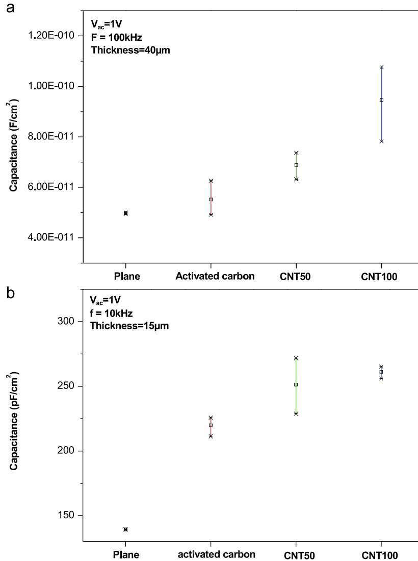
Fig. 4. (a) Capacitance values versus carbonaceous composition for a thickness of 40 \mu\text{m} of polyethylene, for four electrodes types. (b) Capacitance values versus carbonaceous composition for a thickness of 15 \mu\text{m} of polyethylene, for four electrodes types.
