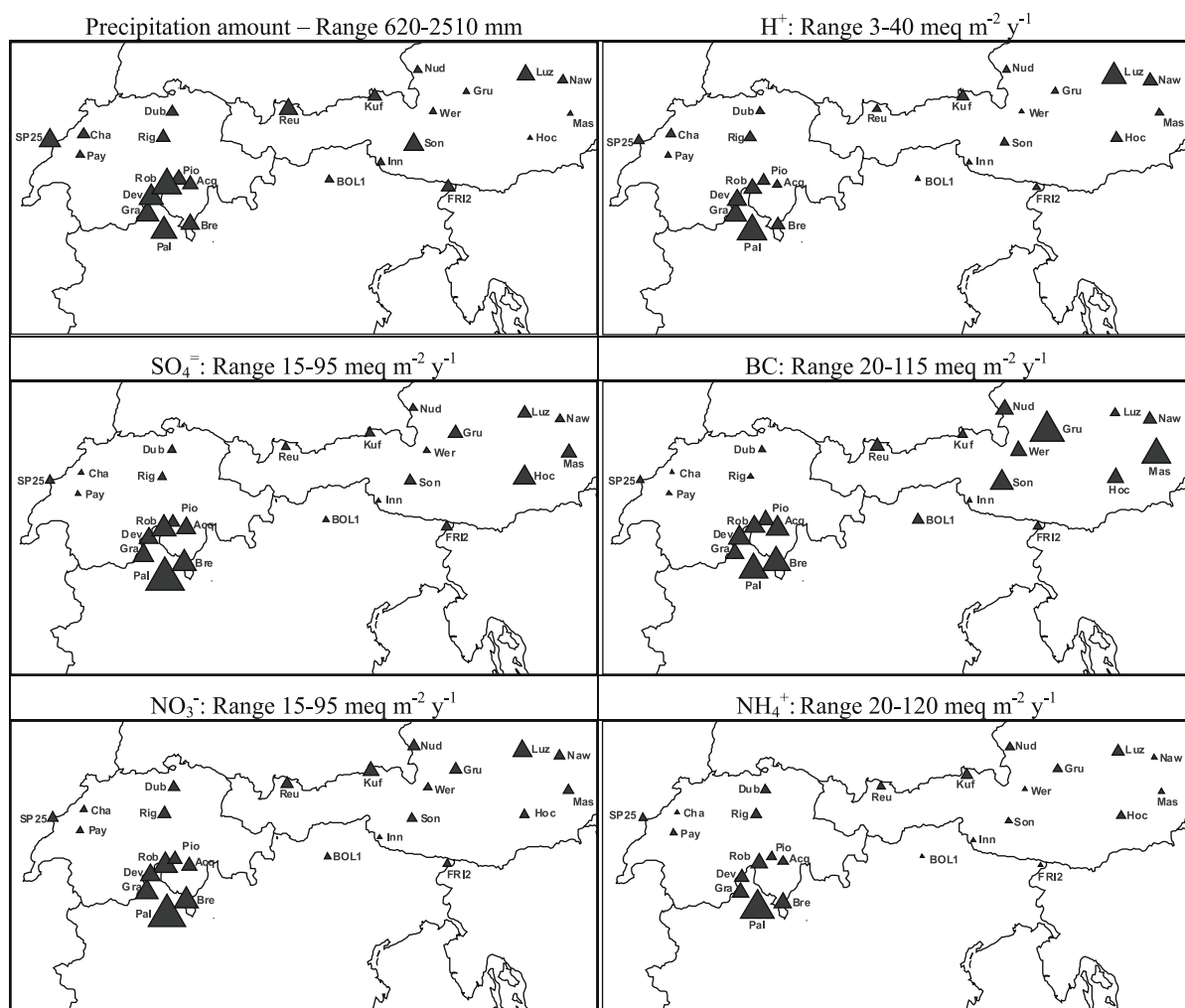
Figure 3. Precipitation amount and fluxes of H^+ , SO_4^{=} , BC (base cations = Ca^{++} + Mg^{++} + Na^+ + K^+ ), NO_3^- and NH_4^+ at wet-only sampling sites (volume weighted mean of 1998–2002). Triangles are proportionally scaled to deposition values. Acronyms as in Table 1.
